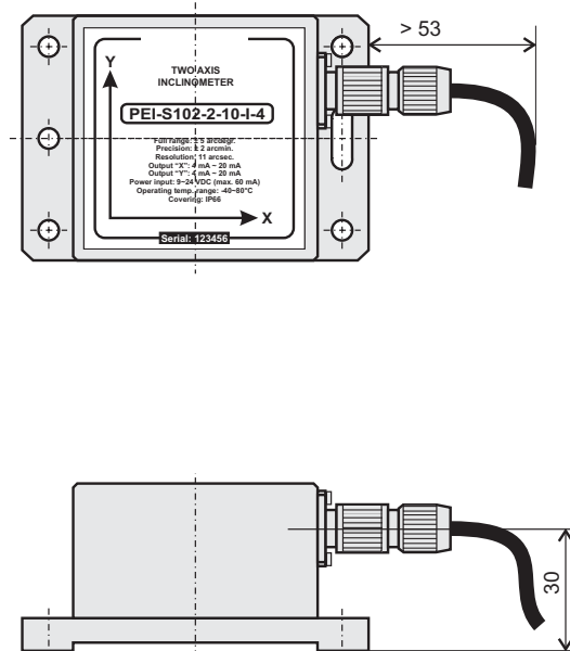
Cover drawing with cable connector (option 4)
