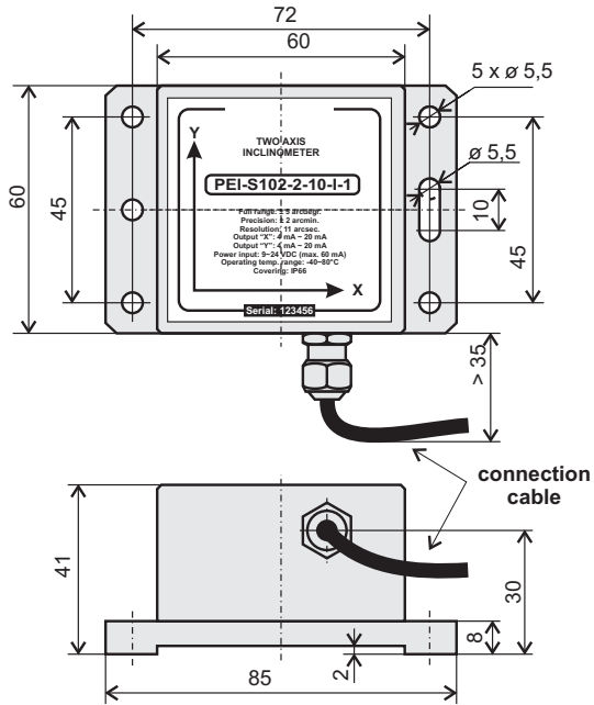
Cover drawing with cable gland (option 1)
