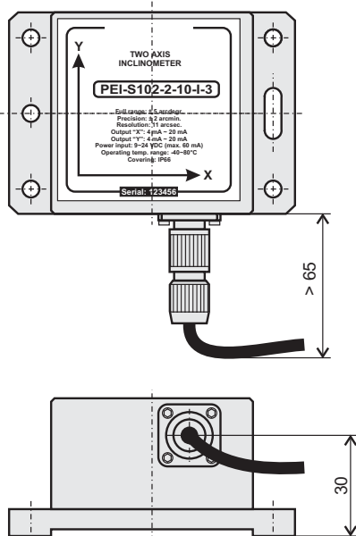
Cover drawing with cable connector (option 3)
